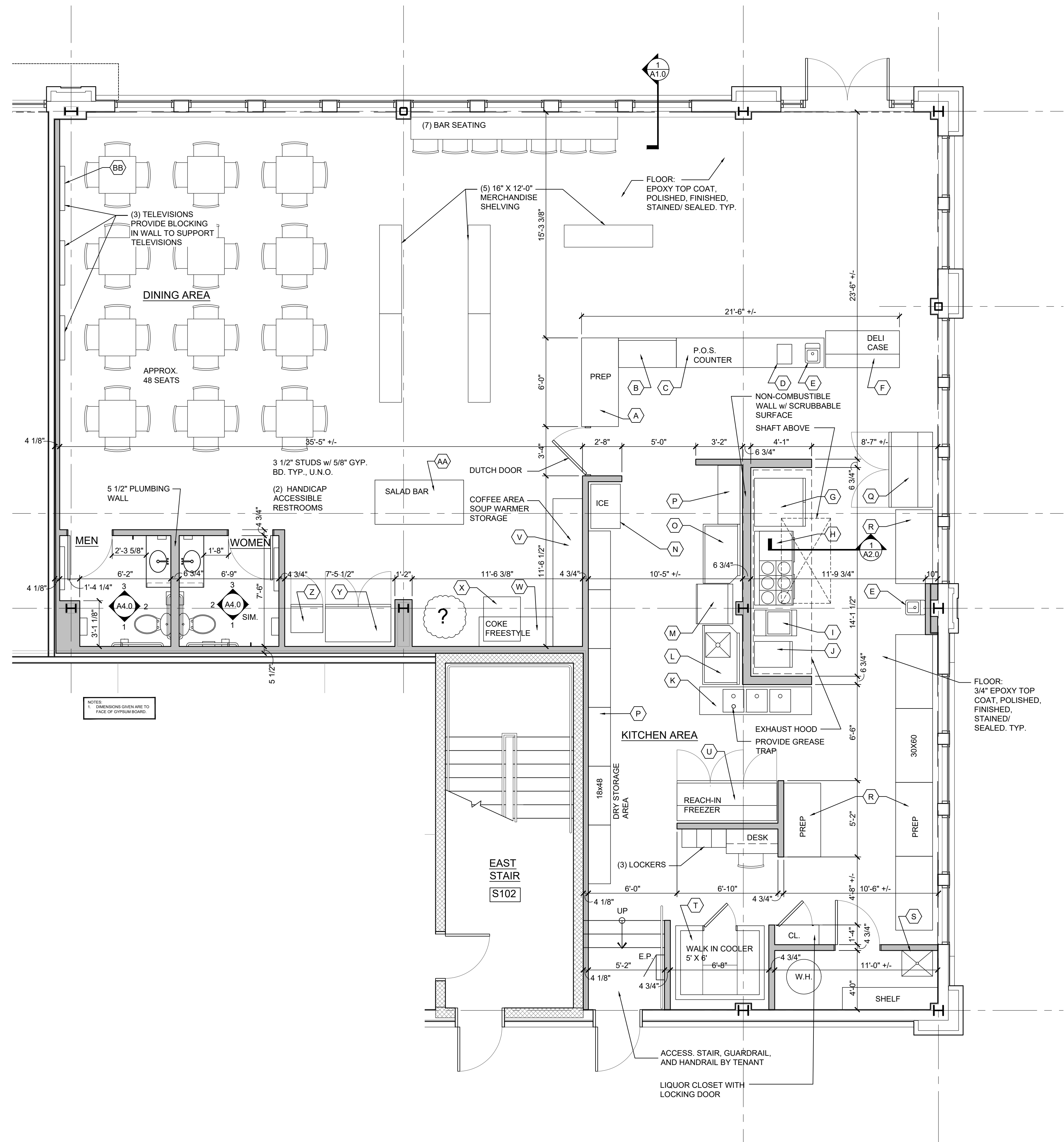
TENANT FLOOR PLAN SCALE: 1/4" = 1'-0"
